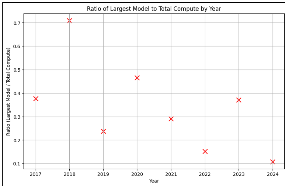
Figure 10: Historical data for the largest model share (LMS) parameter
