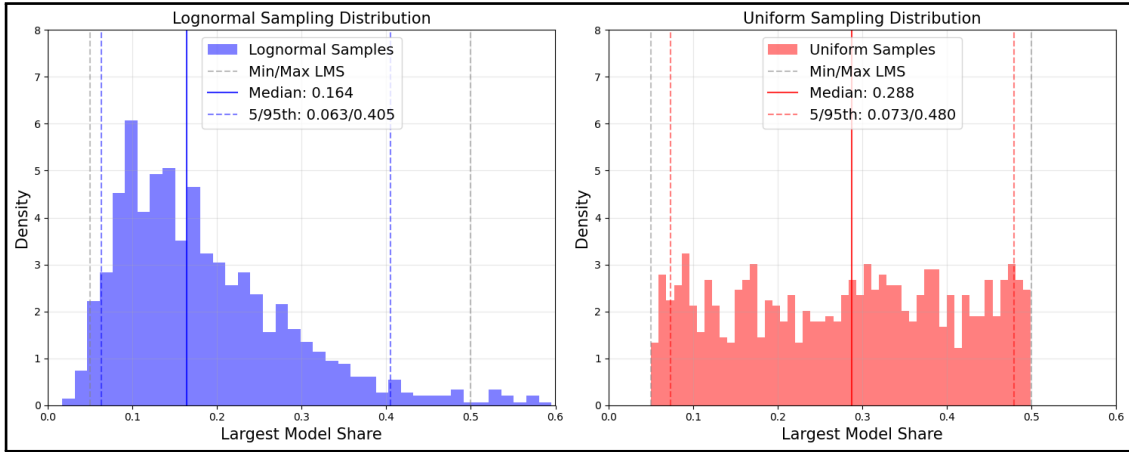
Figure 8: Left: Lognormal LMS distribution with bounds [0.05,0.5] (any value drawn from outside these bounds is resampled) and Right: Uniform LMS distribution. Medians, 5th and 95th percentile LMS indicated.
